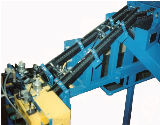
(2) Gravity Ride Rail Tracks to Load Strip Shuttle Unit Shown
