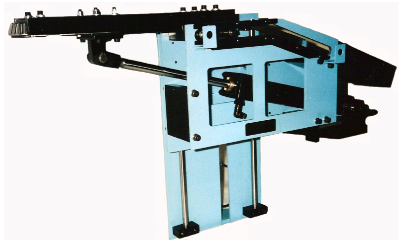
Tapered Bearing Loader into Press Station
